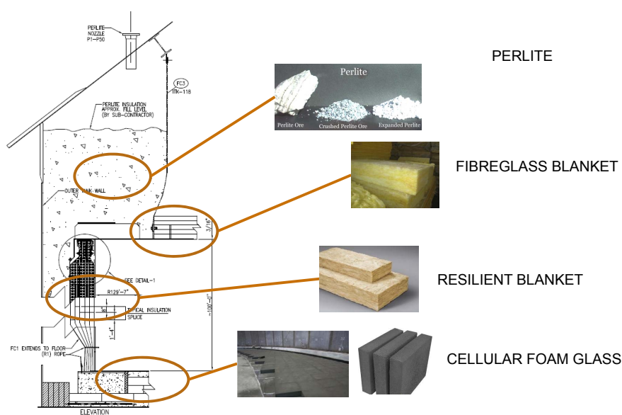
Figure 6. Insulation materials.
