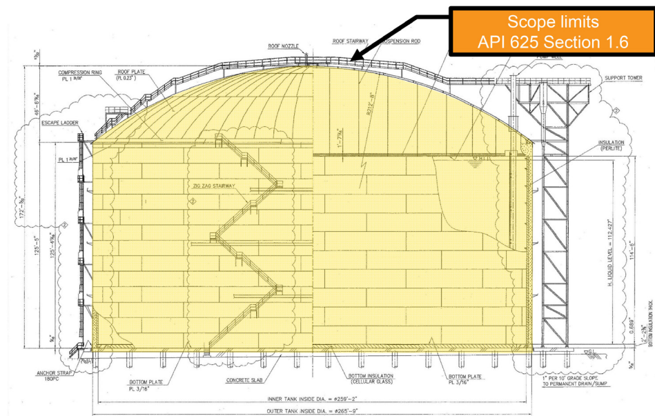
Figure 3. API 625 boundaries.
